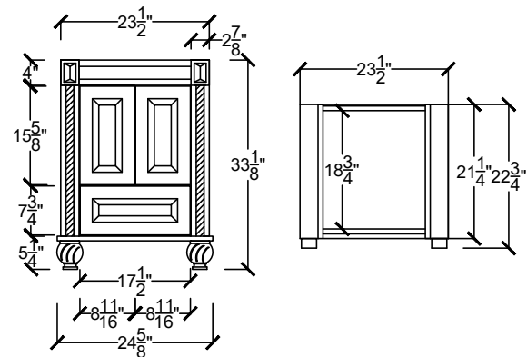
ANAV 2422 BD- - -
